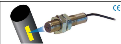
Infrared (1-999,990 RPM) Reliable high speed sensor.
