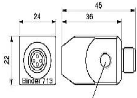
M8 through hole, also for M6 screw
